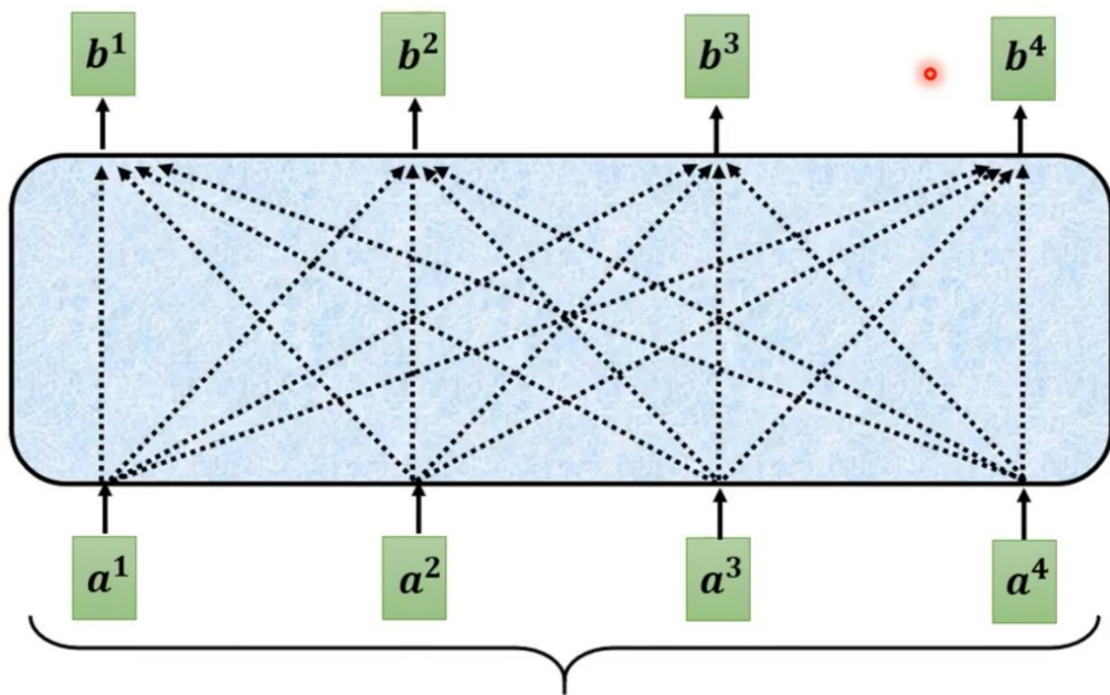
Self attention: 专注于整个序列信息
